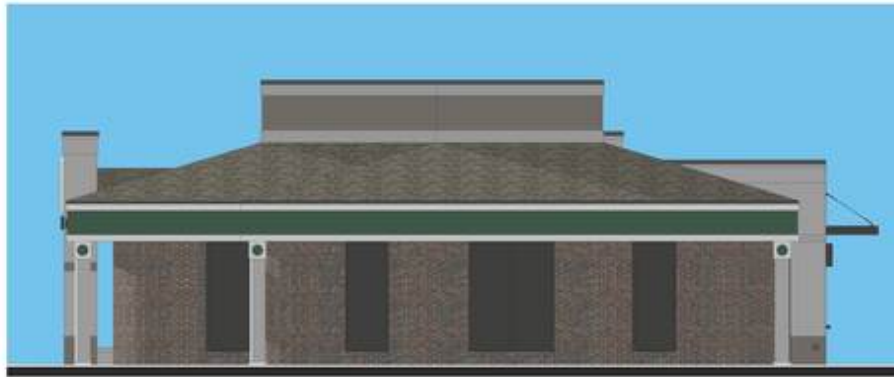
2 NORTH BUILDING ELEVATION SCALE: 1/8"=1'-0"
