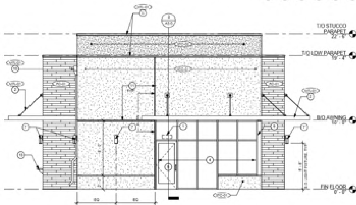
① NORTH ELEVATION 1/4" = 1'-0"
