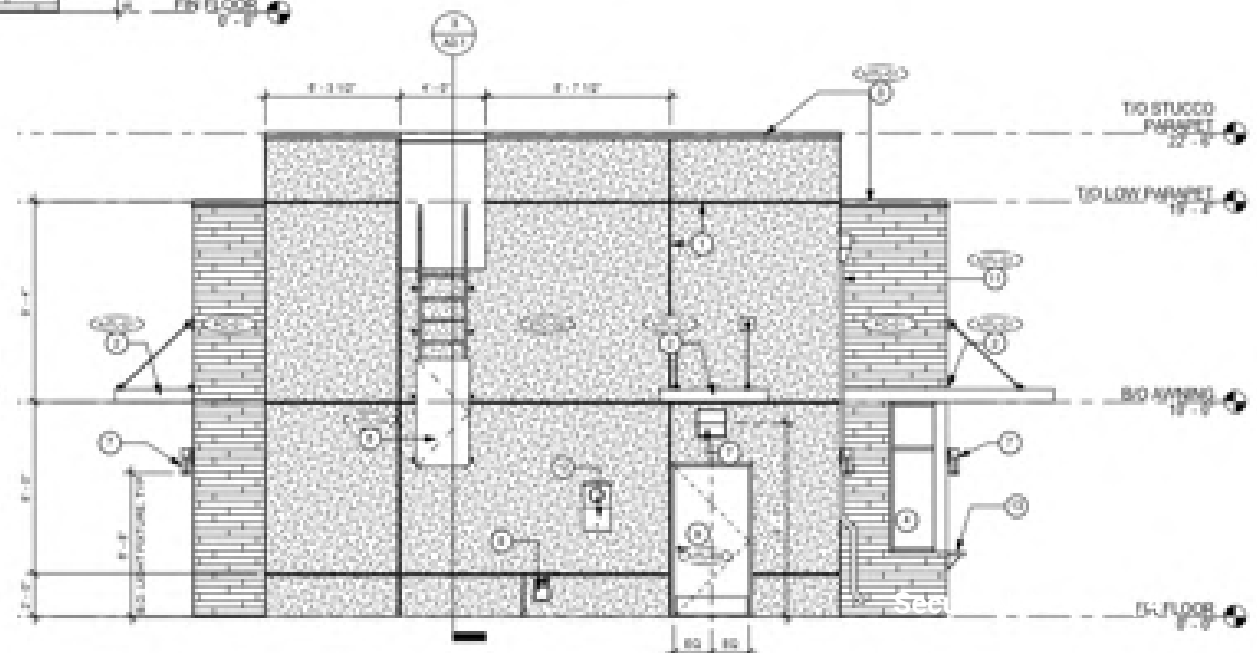
① SOUTH ELEVATION \frac{1}{4}" = 1'-0"
